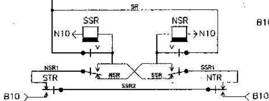
STICK RELAY CIRCUIT USED FOR UNSIGNALLED TRK
